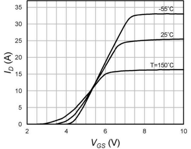
Fig.8 Transfer Characteristics
