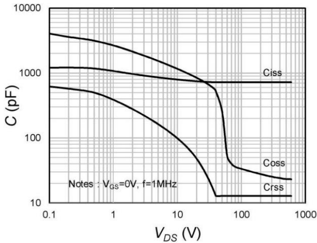
Fig.9 Capacitances
