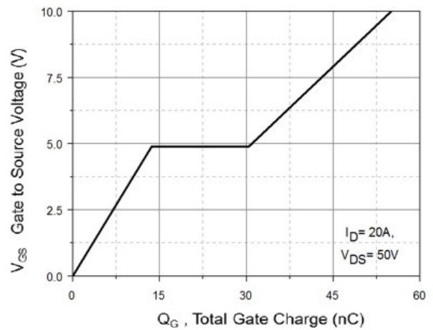
Fig.4 Gate-Charge Characteristics
