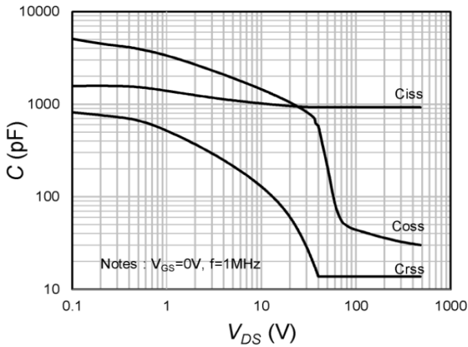
Fig.9 Capacitances
