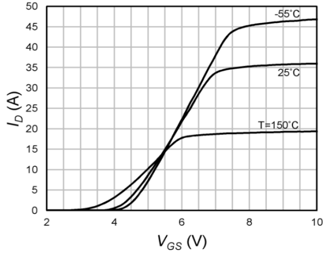
Fig.8 Transfer Characteristics
