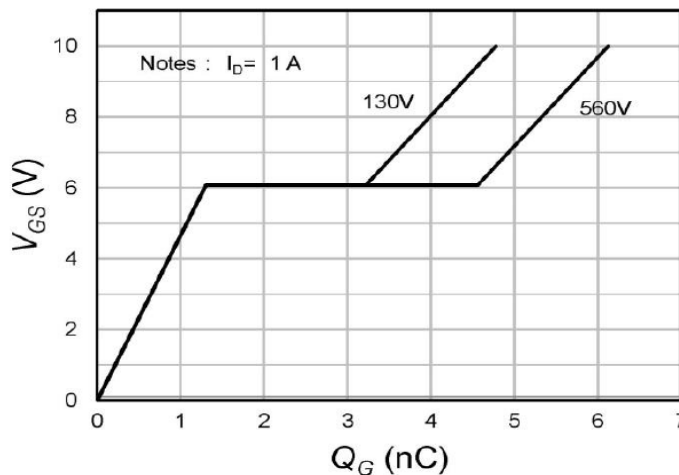
Fig.4 Gate-Charge Characteristics
