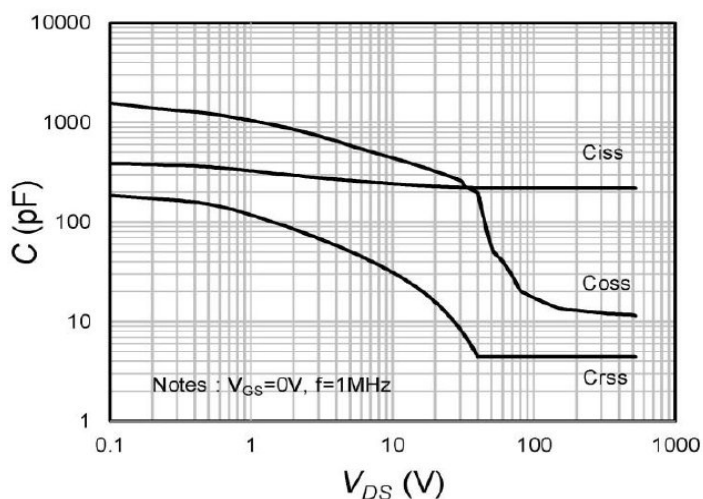
Fig.9 Capacitances
