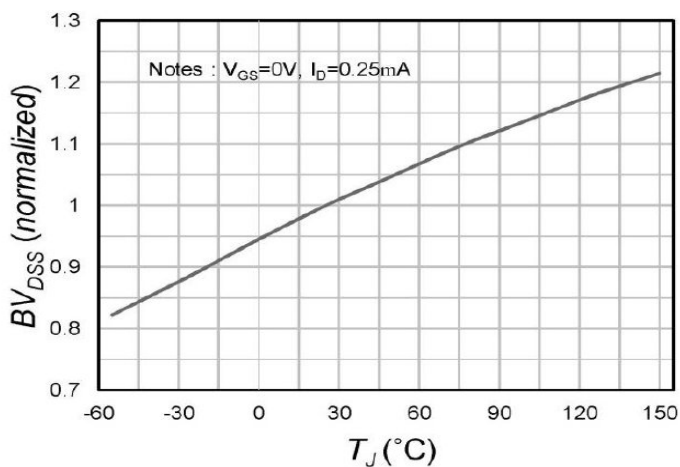
Fig.7 Drain-Source Breakdown Voltage(Normazied)
