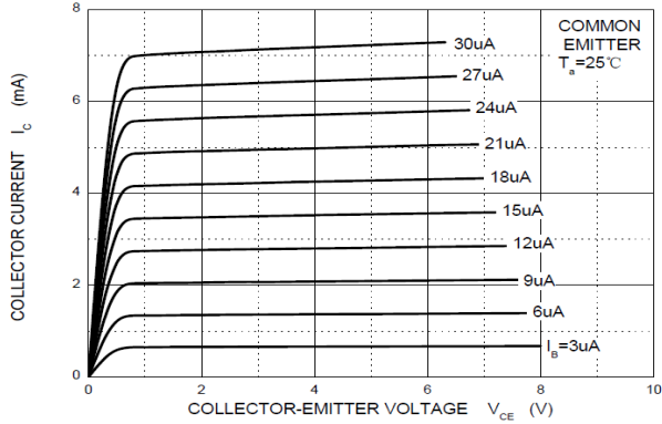
Static Characteristic
