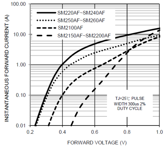
FIG. 2-TYPICAL FORWARD CHARACTERISTICS
