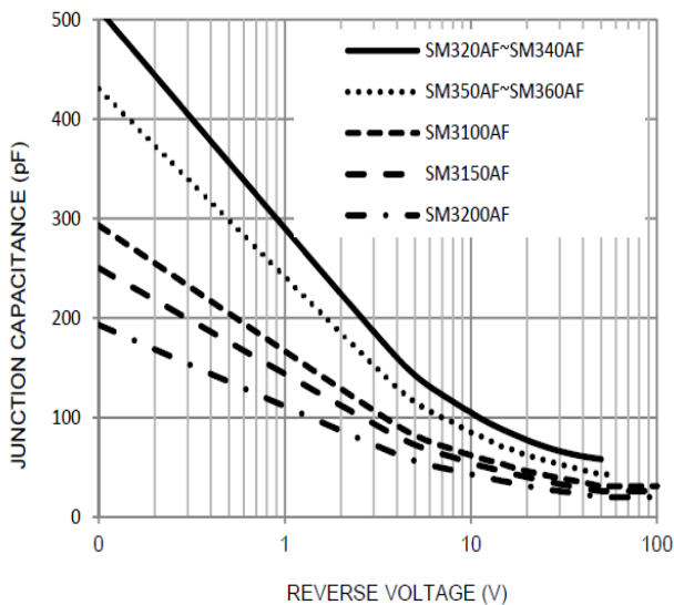
FIG. 5-TYPICAL JUNCTION CAPACITANCE
