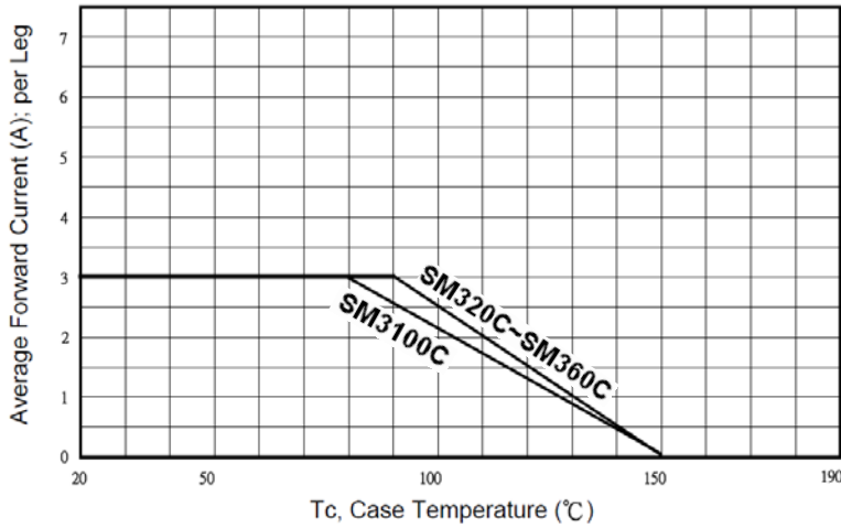
FIG.1-TYPICAL FORWARD CURRENT DERATING CURVE
