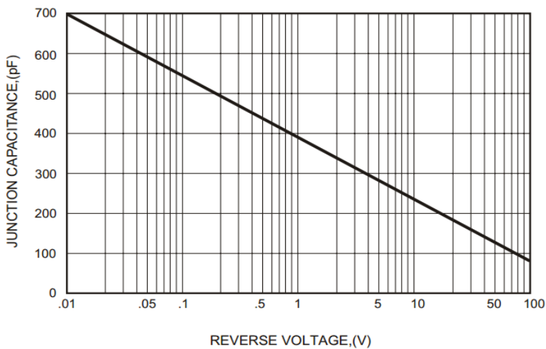
FIG.4-TYPICAL JUNCTION CAPACITANCE
