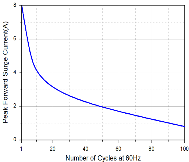
Maximum Non-Repetitive Forward Surge Current
