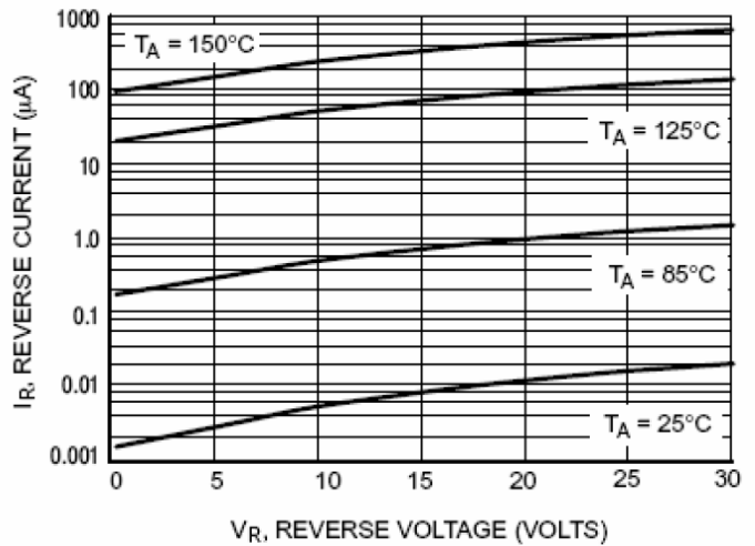
Figure 3. Leakage Current
