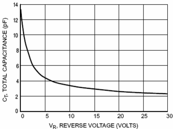
Figure 4. Total Capacitance
