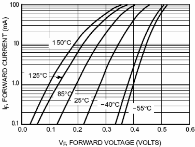
Figure 2. Forward Voltage
