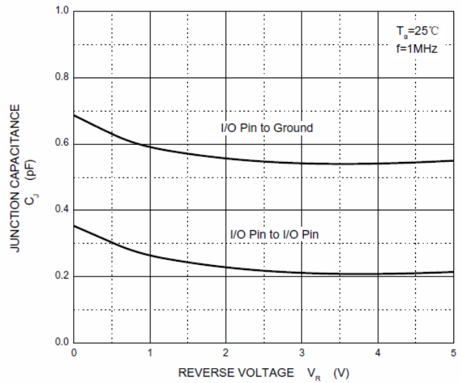
Capacitance Characteristics
