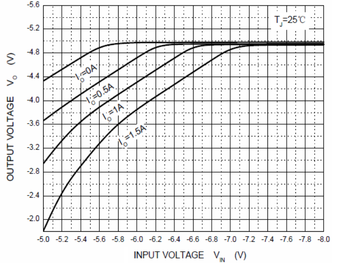
Dropout Characteristics
