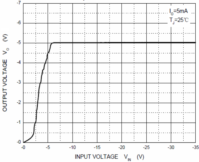
Output Characteristics
