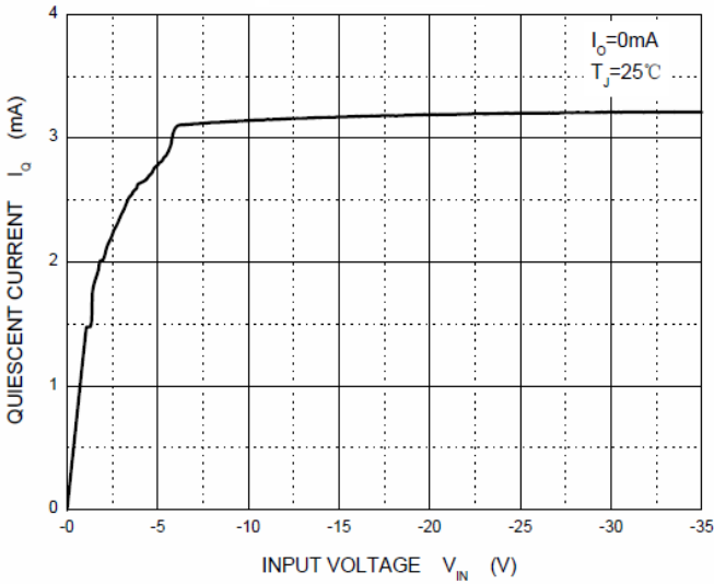
Quiescent Current
