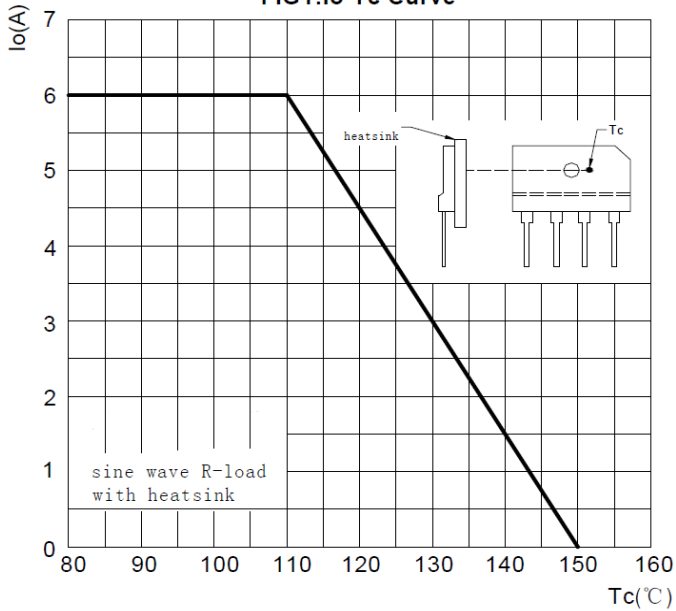
FIG1:Io-Tc Curve
