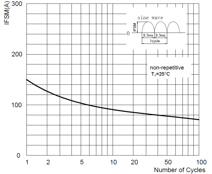
FIG2:Surge Forward Current Capadility
