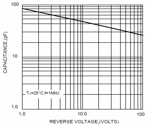
FIG.3-TYPICAL JUNCTION CAPACITANCE
