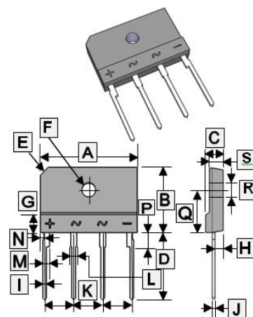
4GBJ
