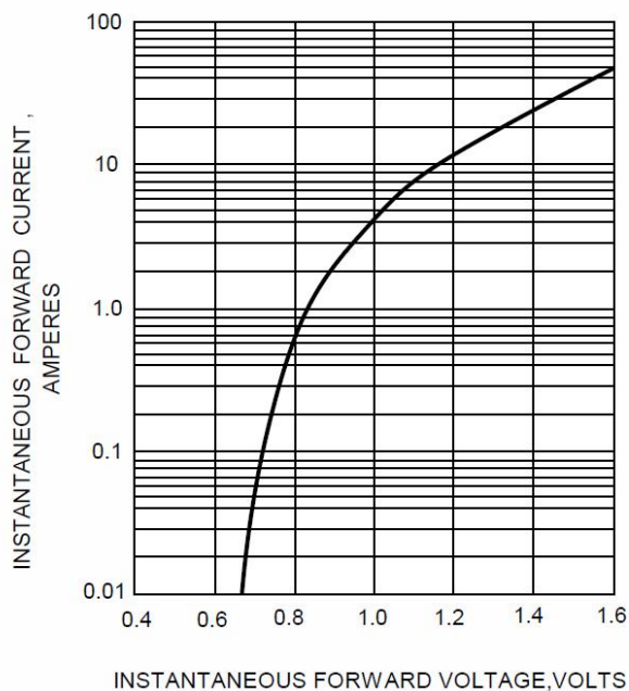
FIG.3-TYPICAL FORWARD CHARACTERISTICS
