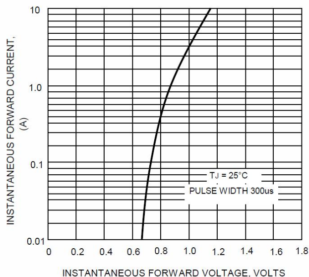
FIG.4-TYPICAL FORWARD CHARACTERISTICS
