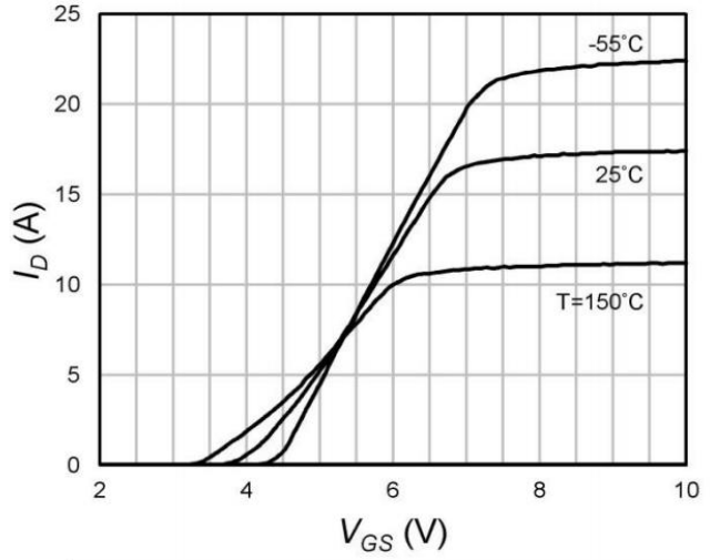
Fig.8 Transfer Characteristics
