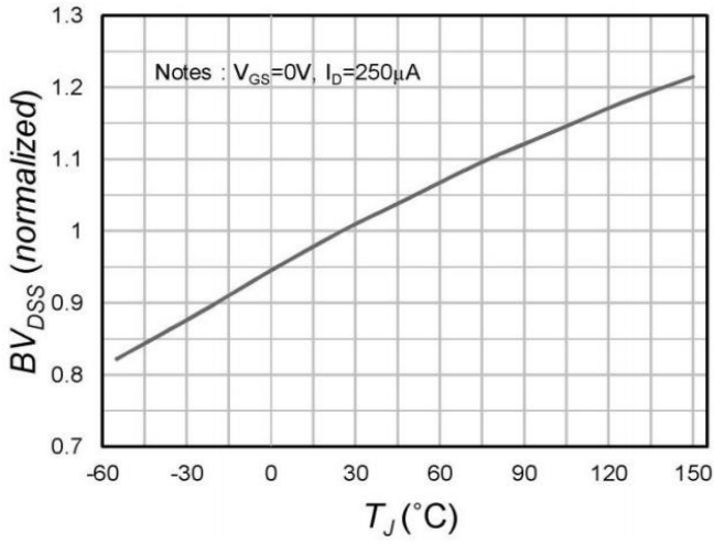
Fig.7 Drain-Source Breakdown Voltage(Normazied)
