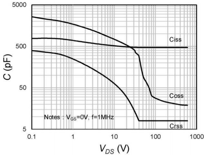
Fig.9 Capacitances
