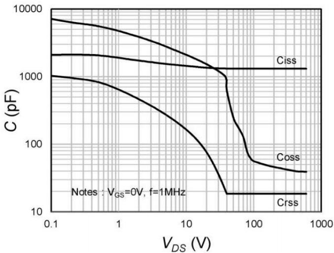
Fig.9 Capacitances
