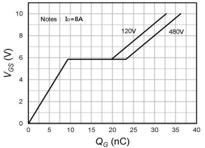
Fig.4 Gate-Charge Characteristics
