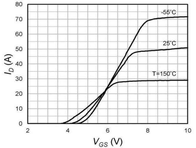
Fig.8 Transfer Characteristics
