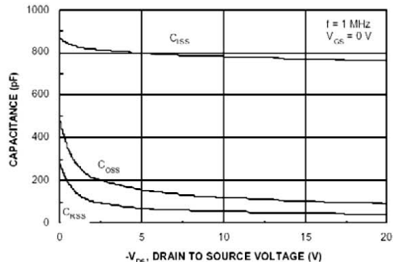
Figure 8. Capacitance Characteristic
