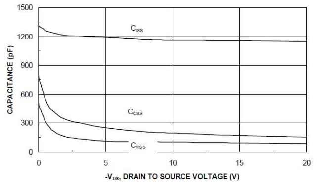
Figure 4. Capacitance
