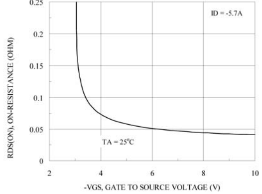
Figure 8. On-Resistance with Gate to Source Voltage
