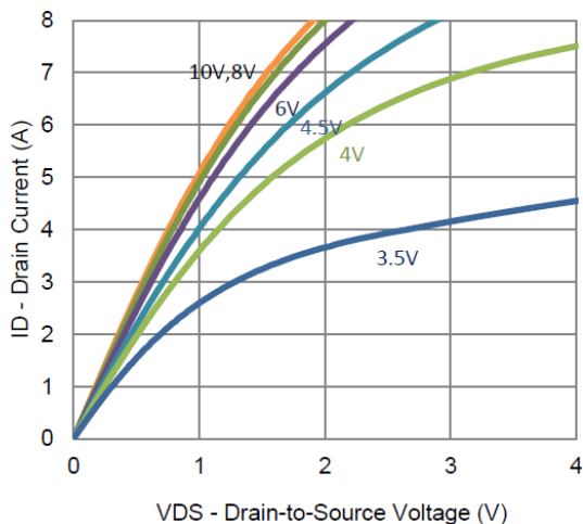
5. Output Characteristics
