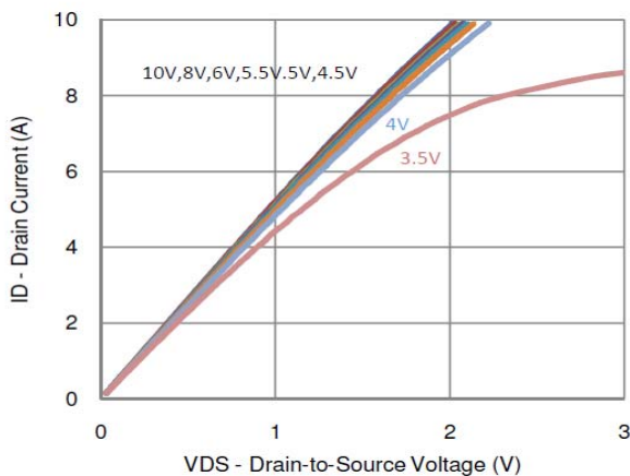
5. Output Characteristics
