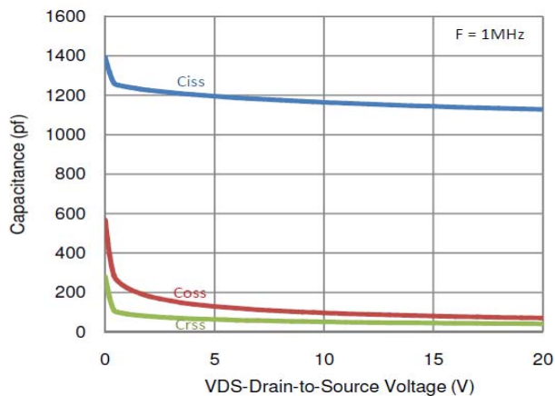
6. Capacitance
