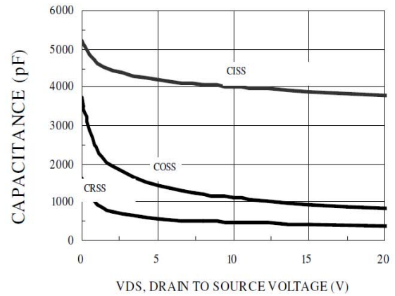
Figure 4. Capacitance
