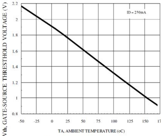
Figure 9. Threshold Voltage
