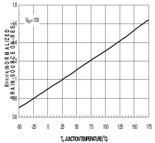
Figure 6. On-Resistance vs. Junction Temperature
