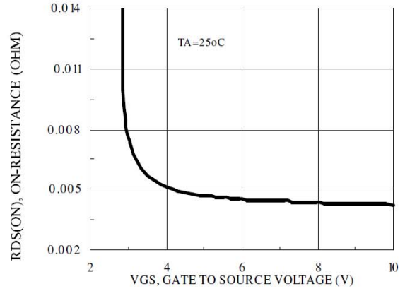
Figure 8. On-Resistance vs. Gate-to-Source Voltage
