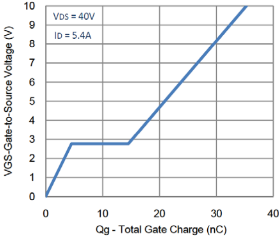
7. Gate Charge
