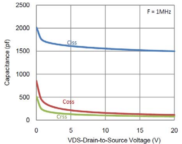
6. Capacitance
