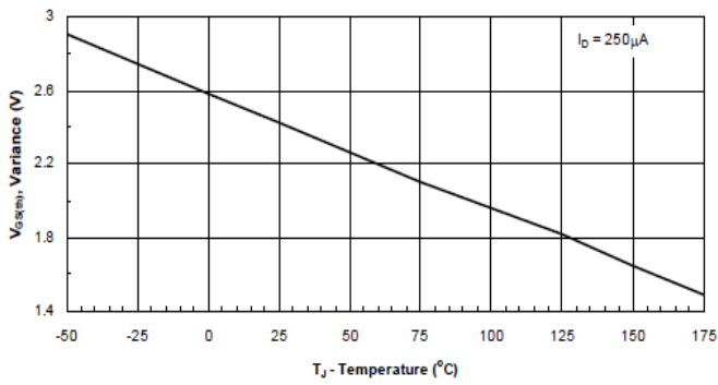
Threshold Voltage
