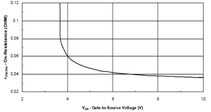
On-Resistance vs. Gate-to-Source Voltage
