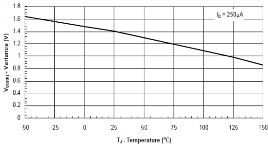
Threshold Voltage
