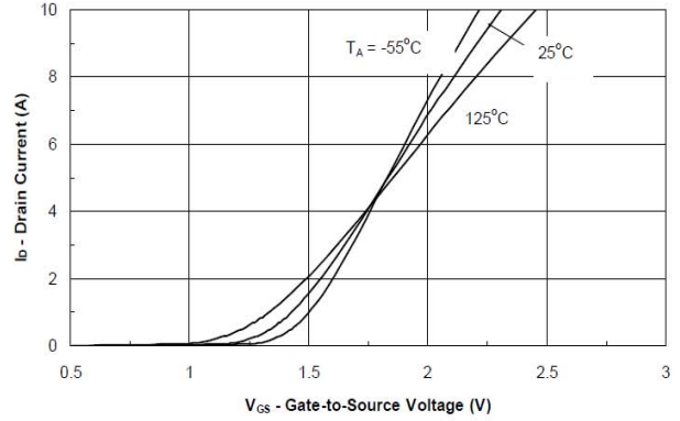
Transfer Characteristics
