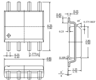
SOP-8
