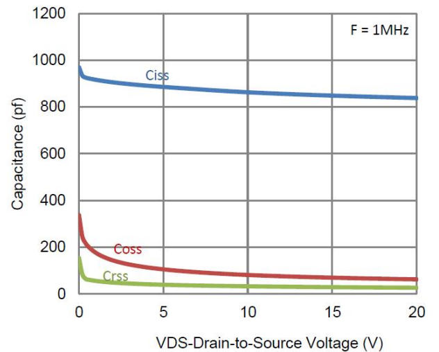
6. Capacitance
