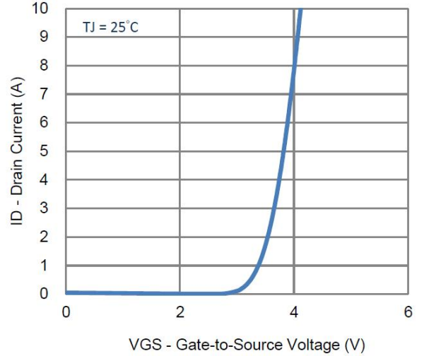
2. Transfer Characteristics
