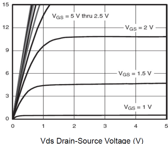
Figure 5 Output Characteristics
