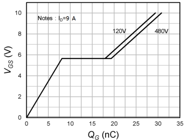
Fig.4 Gate-Charge Characteristics
