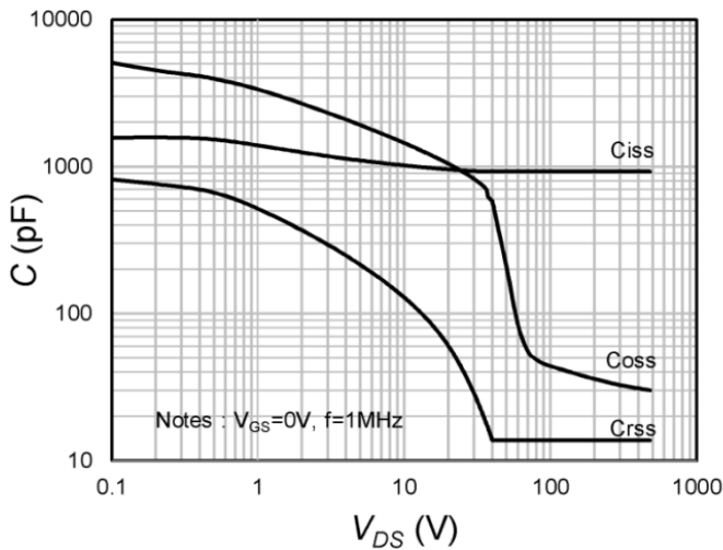
Fig.9 Capacitances
