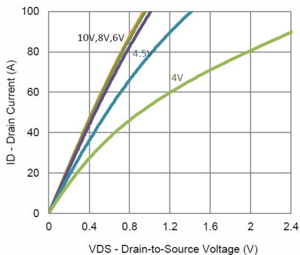
5. Output Characteristics
