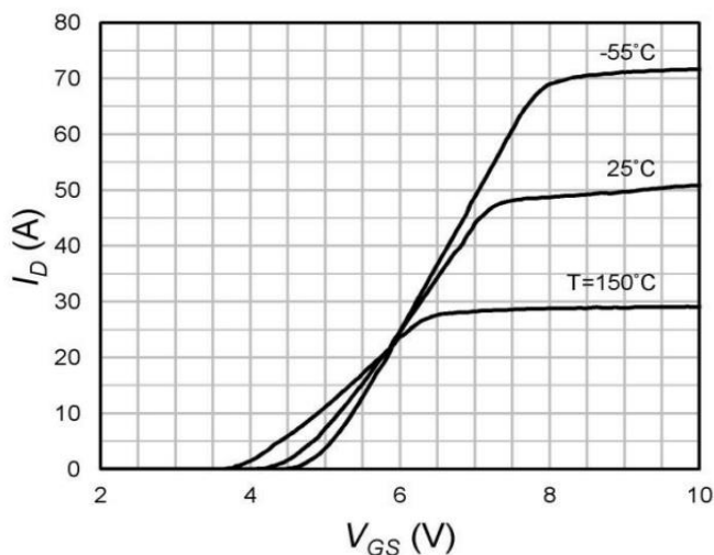
Fig.8 Transfer Characteristics
