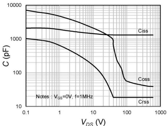
Fig.9 Capacitances
