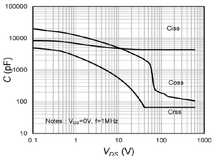
Fig.9 Capacitances
