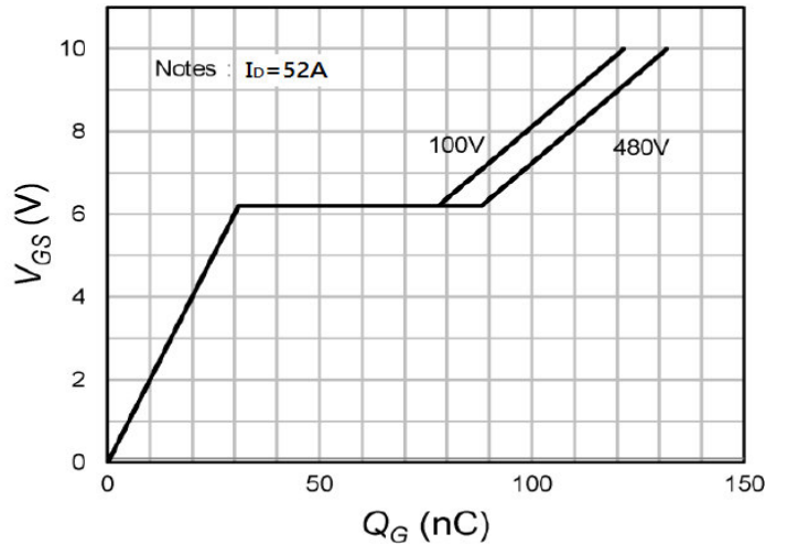
Fig.4 Gate-Charge Characteristics
