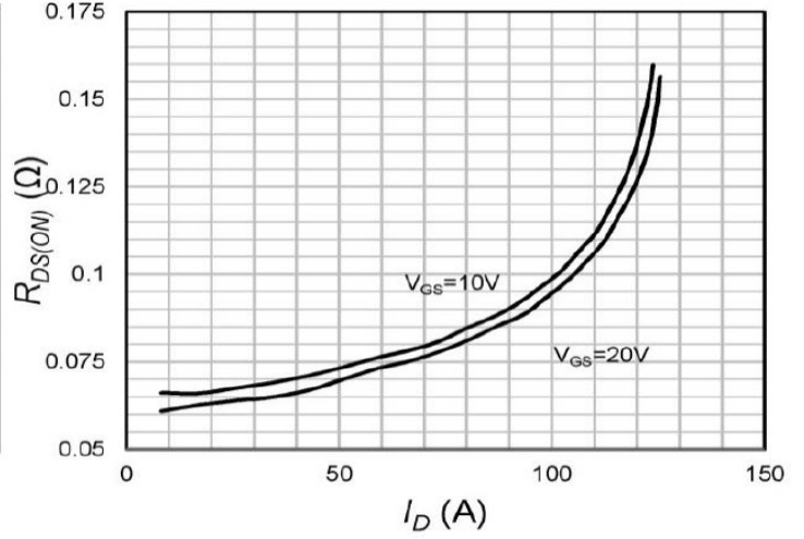
Fig.2 On-Resistance vs. Drain Current
