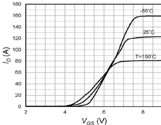
Fig.8 Transfer Characteristics
