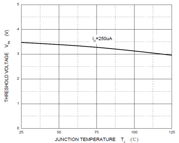
Threshold Voltage
