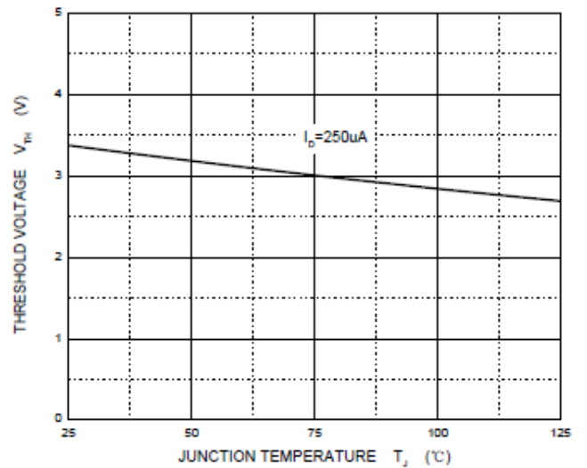
Threshold Voltage
