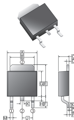
TO-252
