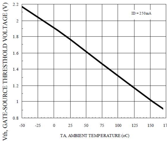
Figure 9. Threshold Voltage
