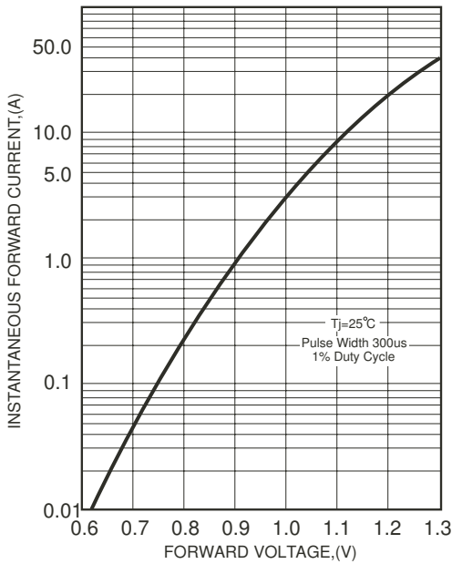
FIG.1-TYPICAL FORWARD CHARACTERISTICS
