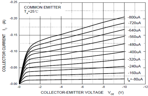
Static Characteristic
