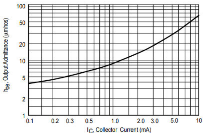
Figure 12. Output Admittance
