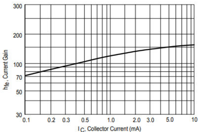
Figure 11. Current Gain
