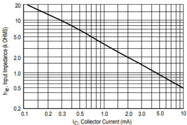
Figure 13. Input Impedance
