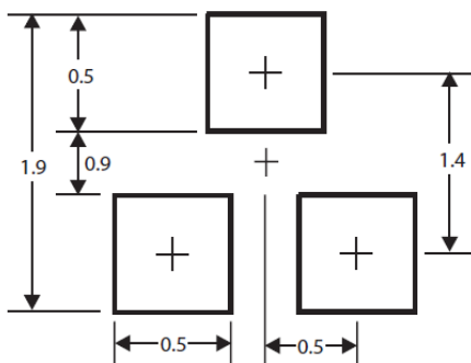
Figure 19. Mounting Pad Layout
