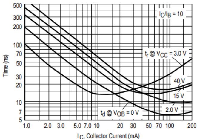
Figure 5. Turn-On Time
