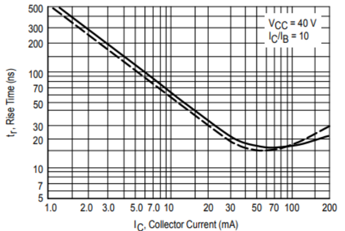
Figure 6. Rise Time
