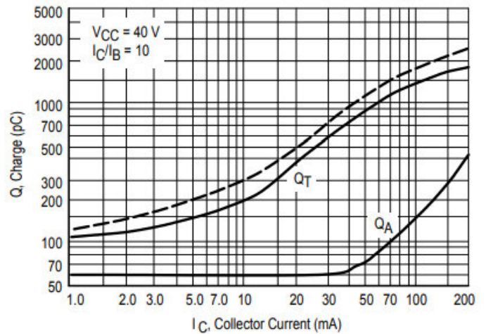
Figure 4. Charge Data
