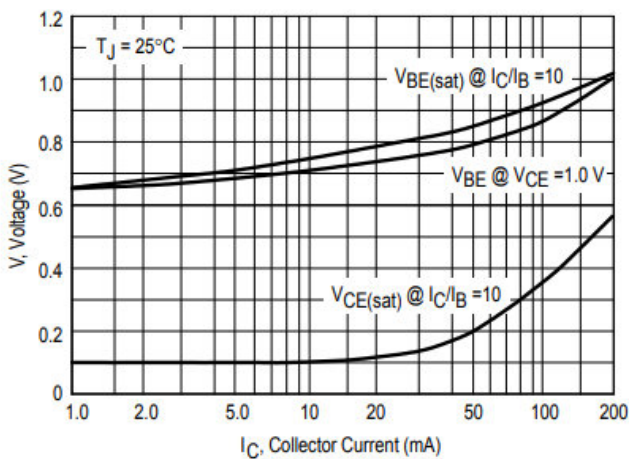
Figure 17. "ON" Voltages
