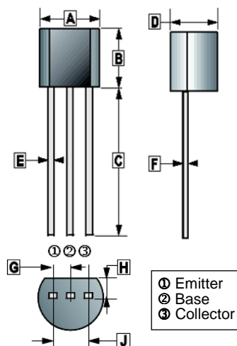
TO-92
