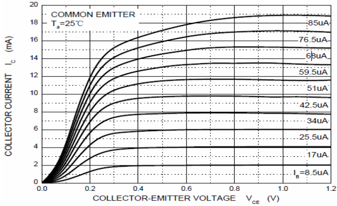
Static Characteristic
