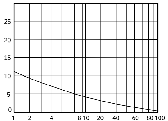
FIG .5-PEAK FORWAED SURGE CURRENT
