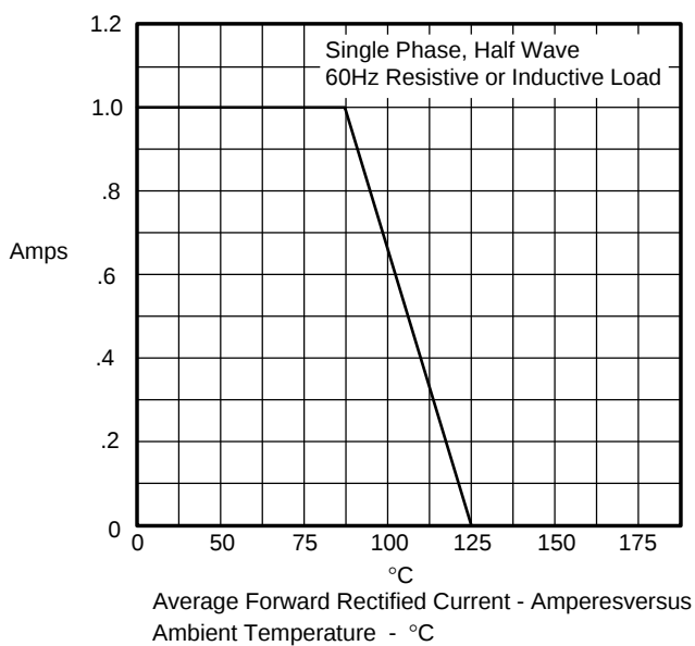
FIG.3-FORWARD DERATING CURVE
