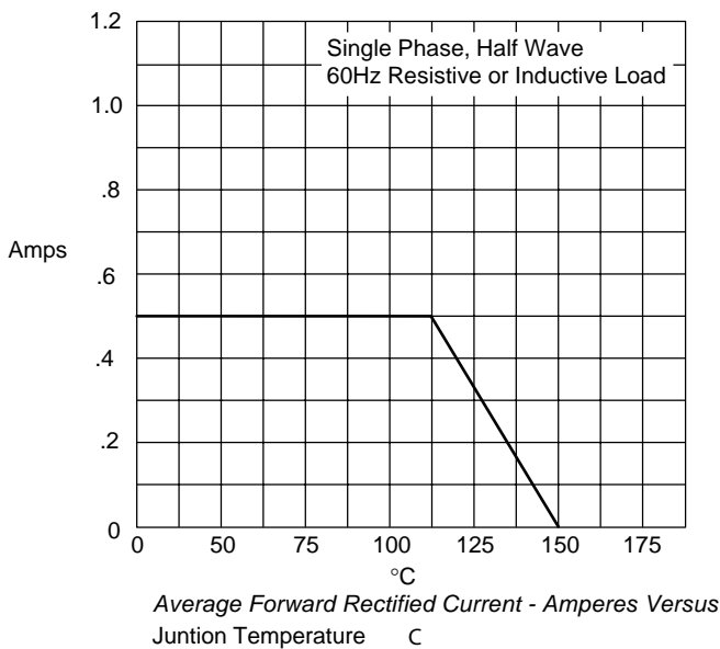
FIG.3-FORWARD DERATING CURVE
