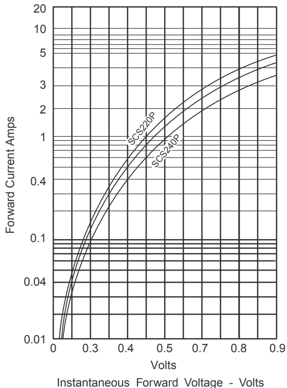
FIG.1-TYPICAL FORWARD CHARACTERISTICS
