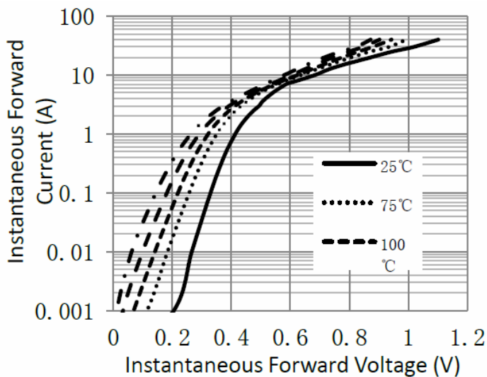
Figure 3. Typical Instantaneous Forward Characteristic
