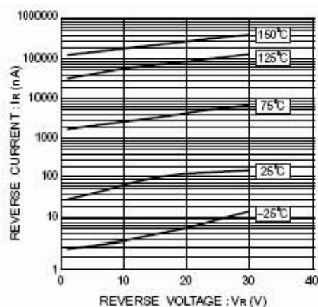
Fig.2 Reverse characteristics
