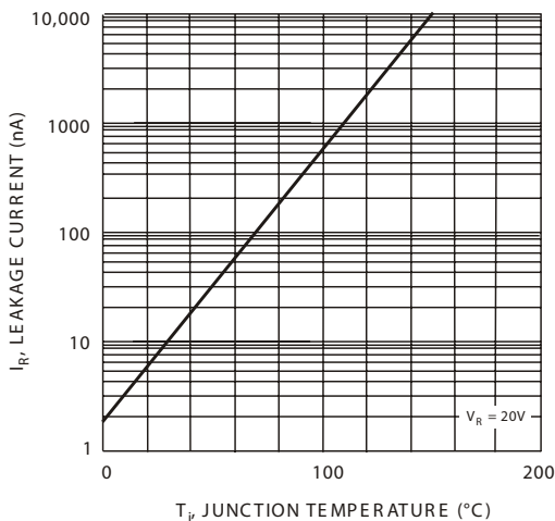
Fig. 3 Leakage Current vs Junction Temperature
