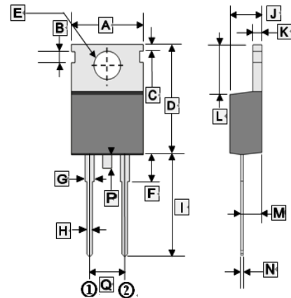
TO-220YA
