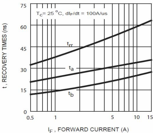
FIG.5 - T rr , t a AND t b CURVES vs FORWARD CURRENT
